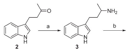
Scheme 1. Synthesis of Racemic 1
