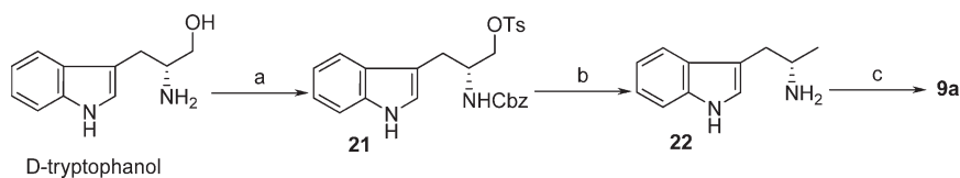
Scheme 3. Synthesis of the Active Enantiomer of 9a from D-Tryptophanol
